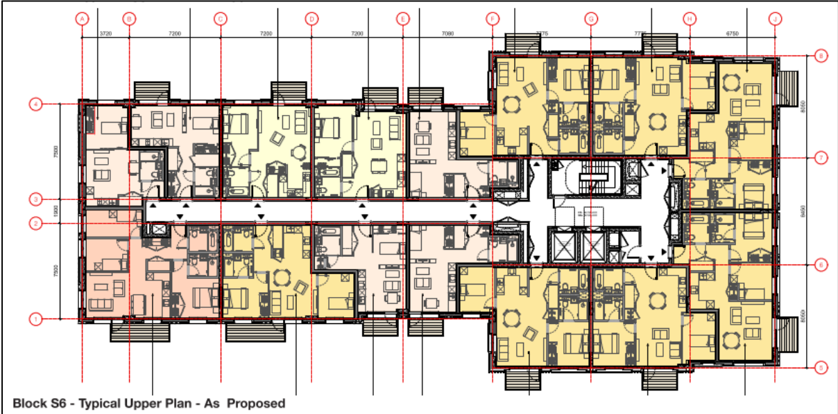
Typical upper floor plan Building S6 as proposed – 15 dwellings
